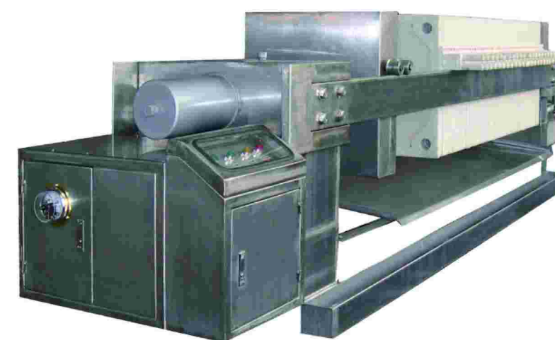
带接液槽板框式压滤机 Plate & frame filter press with flume
