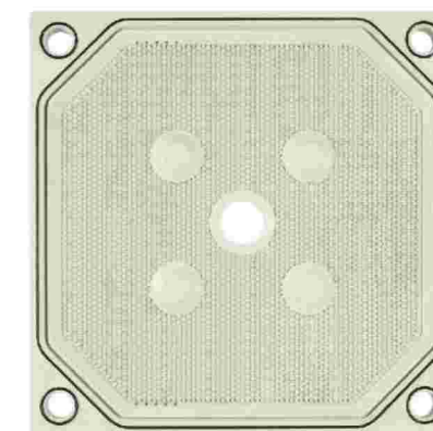
带密封条滤板 Filter plate with sealing
