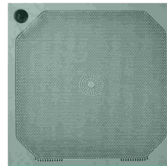
角进料聚丙烯隔膜滤板 PP membrane corner feed plates
