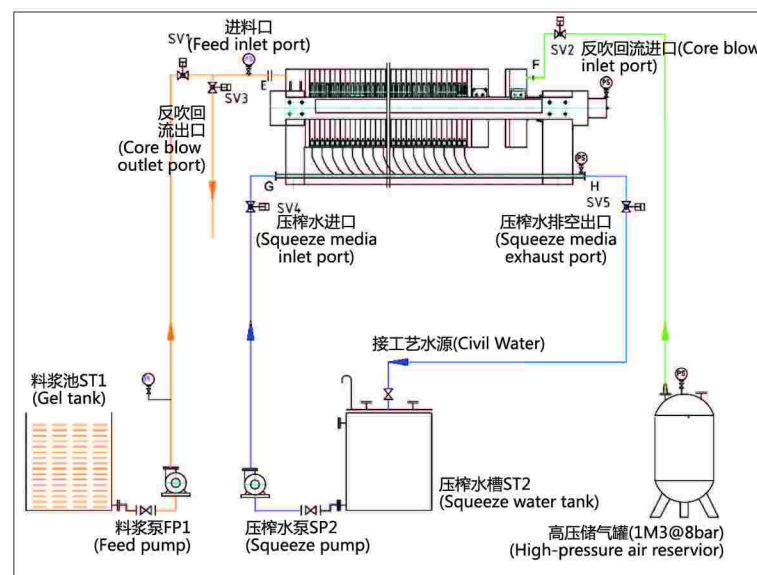
典型的安装图 Typical layout plan
