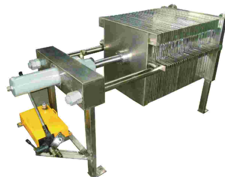
手动型不锈钢压滤机 Manual filter press with SS filter plate
