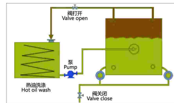
热油洗涤过程 Hot oil washing cloth process
