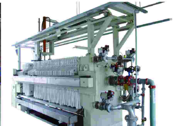
▲ 转90° 滤布清洗 turn 90° for cloth wash
